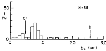
Fig. 10 Frequency histogram of transverse displacement of suspended particles.
