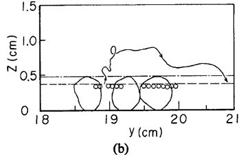
Fig. 9(a), (b) Typical profiles of trajectories projected on y-z plane.
