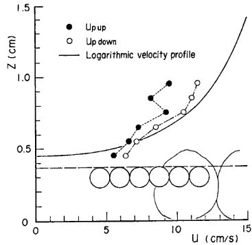
Fig. 8 Vertical profiles of the longitudinal velocity of the particles which move upward and downward.
