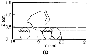
Fig. 9(a), (b) Typical profiles of trajectories projected on y-z plane.
