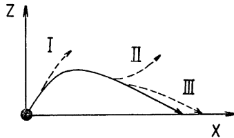
Fig. 19 Process of a particle motion transforming into suspension from saltation.
