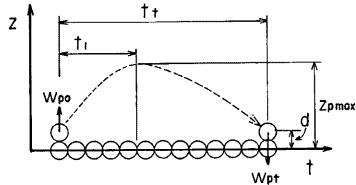
Fig. 16 Coordinate system and symbols.
