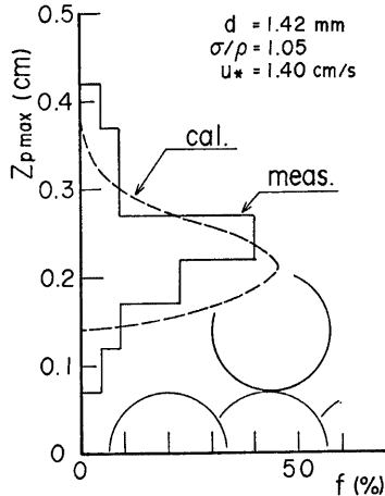
Fig. 18 Comparison between the theoretical result and the experimental one for the probability density distribution of the maximum level of position at which salting particles terminate upward motion.
