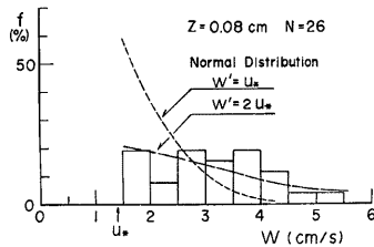
Fig. 12 Frequency histogram of vertical fluid velocity which was obtained from eq. of a particle motion and its trajectory.
