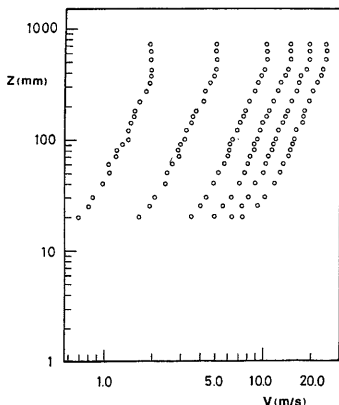
Fig. 3 Mean velocity profile of wind model
