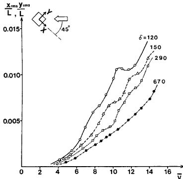
Fig. 8-c RMS responses in y (or x ) direction of the model for different values of mass-damping parameters ( \alpha=45^\circ )
