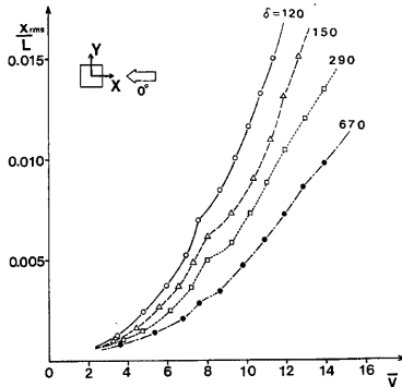
Fig. 8-d RMS responses in x direction of the model for different values of mass-damping parameters ( \alpha=0^\circ )
