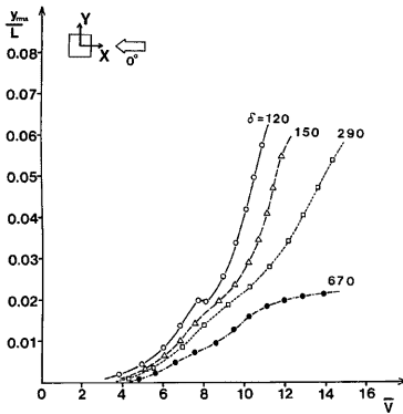
Fig. 8-a RMS responses in y direction of the model for different values of mass-damping parameters ( \alpha=0^\circ )
