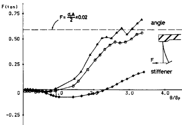
Fig. 12 Bracing force in stiffener and angle- brace
