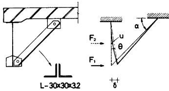
Fig. 16 Estimation of the bracing rigidity of the angle-brace
