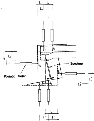
Fig. 5 Method of displacement measurement
