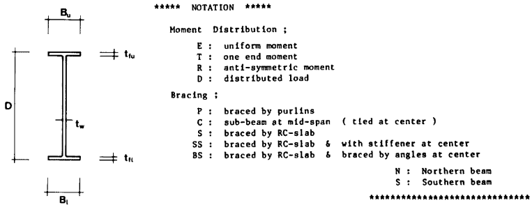
Fig. 3 Notation in dimensions of the beam
