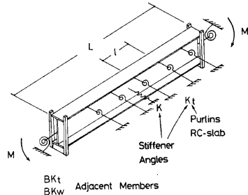
Fig. 13 Analytical model in FEM analysis
