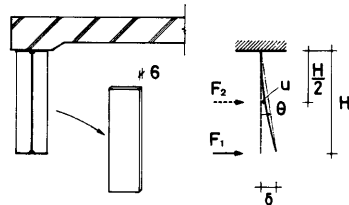
Fig. 15 Estimation of the bracing rigidity of the stiffener
