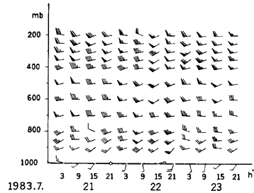
Fig. 4 Vertical time section of winds (a long bard 10 knots) from 21 to 23 July, 1983, over Yonago
