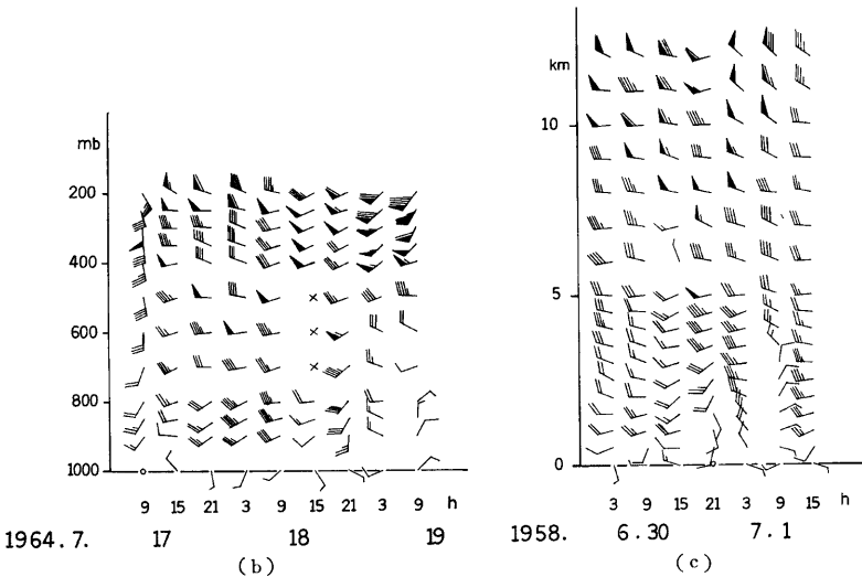
Fig. 10 The same as Fig. 4, but for, (a) 10-13 July, 1972, (b) 17-19 July, 1964, and (c) 30 June-1 July, 1958
