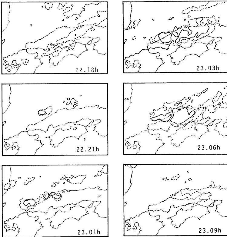
Fig. 8 Areas with blackbody temperature lower than -50^{\circ}\text{C} from 18 h (JST) on 22 to 9 h on 23, July, 1983, broken contour line : -50^{\circ}\text{C} , inner contour line : -60^{\circ}\text{C} , black area : lower than -70^{\circ}\text{C}
