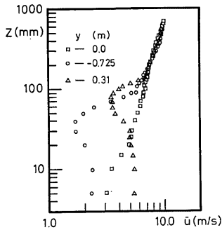
Fig. 2 (e) Mean speed profiles at various locations: U=10.0 m/s, x=9.6 m
