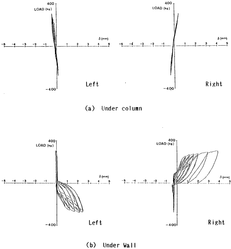
Fig. 10 Load-Vertical displacement relationships of static test
