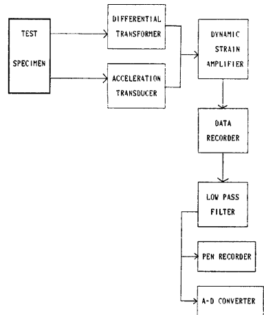
Fig. 7 Flow of measurements of dynamic rest
