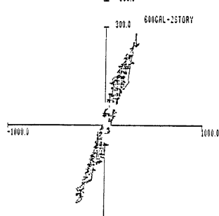
Fig. 13 Responses of model subjected to 600 gal input
