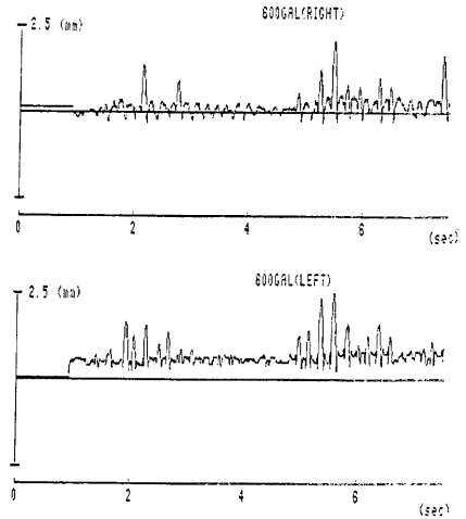
Fig. 15 Time history of vertical displacement
