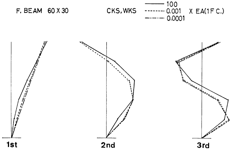
Fig. 18 Effect of soil condition on the mode shape
