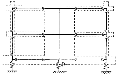
Fig. 11 Analytical model for test frame
