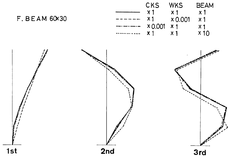
Fig. 19 Effect of boundary condition on the mode shape
