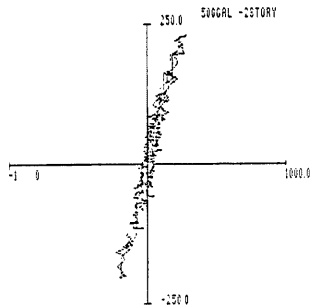
Fig. 12 Responses of model subjected to 500 gal input
