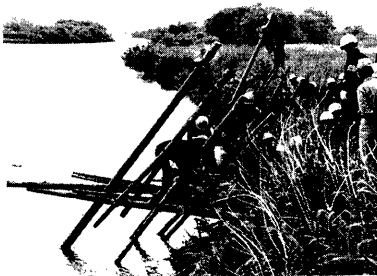
Photo 2 Kawakura in the Jintsu River (during a flood fighting drill)
