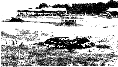
Photo 7 Kamadan ko (circular hooping by sandbags) in the Yodo River (during a flood fighting drill)
