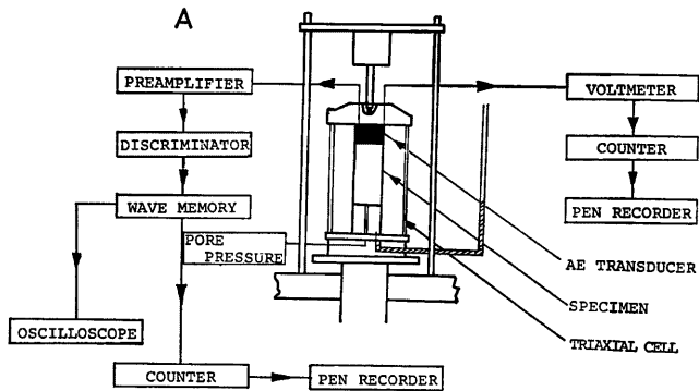
Fig. 4 Block diagram of AE- and triaxial- apparatus
