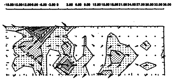
Fig 5 Cross section of the slip distribution in the fault plane. The two segments are connected in the figure. The left 18km fault length is for the Awaji segment and the rest (right 36 km length) is for the Kobe segment. Arrows indicate slip vector directions and relative amplitudes for each subfault.
