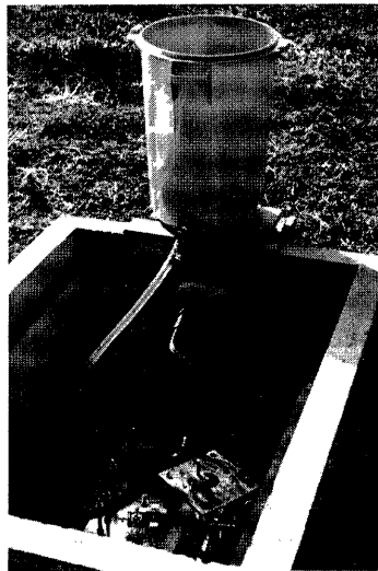
Photo 7 Apparatus for replacing a mixture of water and ethylene glycol by distilled water.
