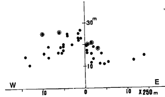
Fig. 2 Distribution of elevations which are measured along the lines across the fault. Vertical axis indicates height in m unit and horizontal one indicates distance in m unit.
