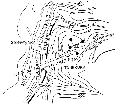
Fig. 4 Topographical map near the Miyagawa observation site and the location of electrodes, where 1-2 and 3-4 show two pairs of electrodes buried under the ground.
