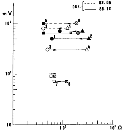
Fig. 8 Relation between electric potential differences and earth resistances of carbon-rod electrodes. 1-2, 3-4, 5-6 and 7-8 show four pairs of electrodes. Each arrow shows the direction of earth currents between each pair of electrodes.
