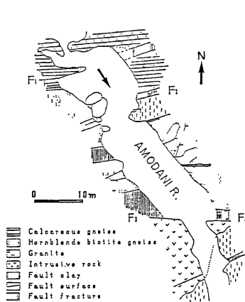
Fig. 3 Geological map of the Amo-valley outcrop on the Atotsugawa fault.
