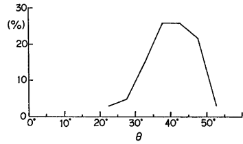
Fig. 9 Distribution of slope failure in the research field.
