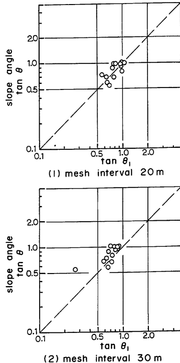
Fig. 11 Comparison of the real slope angle \theta and average one \theta_1 evaluated by mesh method for slided slopes.
