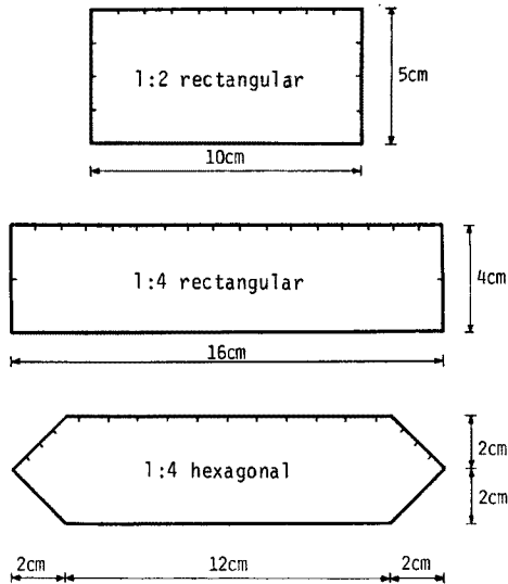
Fig. 2. Cross sections of models.
