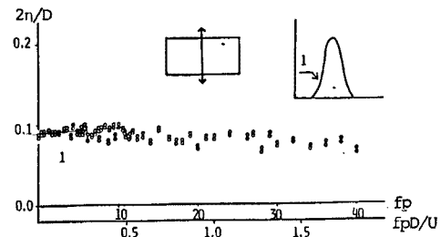
Fig. 20. Heaving response amplitude V. S. pulsating frequency diagram in smooth flow. (1:2 rectangular cylinder, f_0=5.5\text{Hz} )
