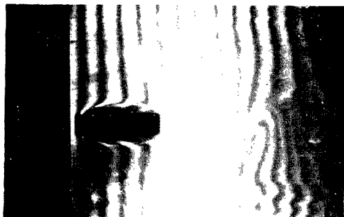
Photo. 3. Flow pattern around 1 : 4 rectangular cylinder in smooth flow. (stationary, Re=0.45 \times 10^4 )
