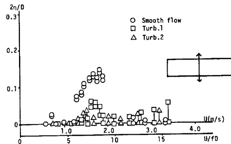
Fig. 18. Heaving response amplitude V. S. wind velocity diagram. (1:4 rectangular cross section)
