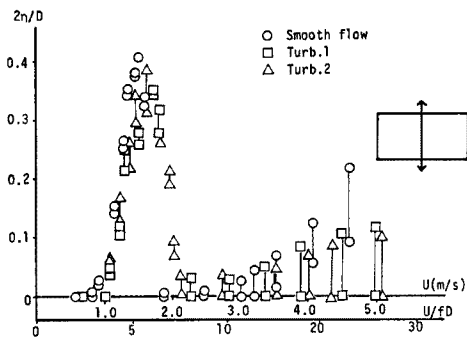
Fig. 17. Heaving response amplitude V. S. wind velocity diagram. (1:2 rectangular cross section)
