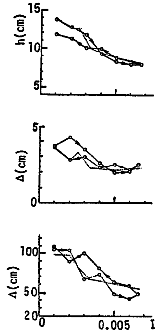
Fig. 6 Histerises of wave length, wave height and flow depth.
