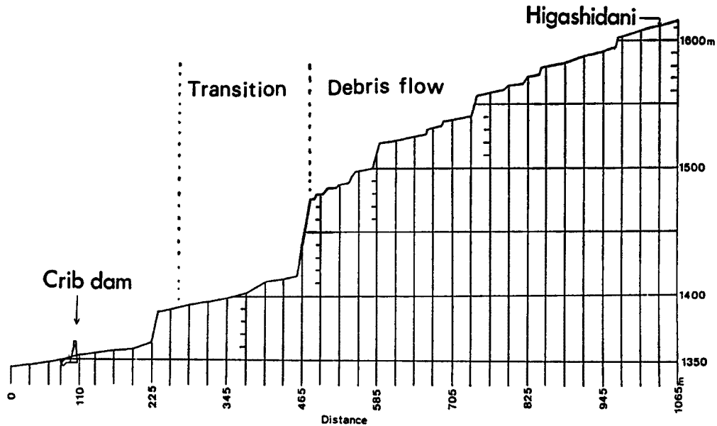
Fig. 18 Longitudinal profile of the Shiramizudani stream channel.
