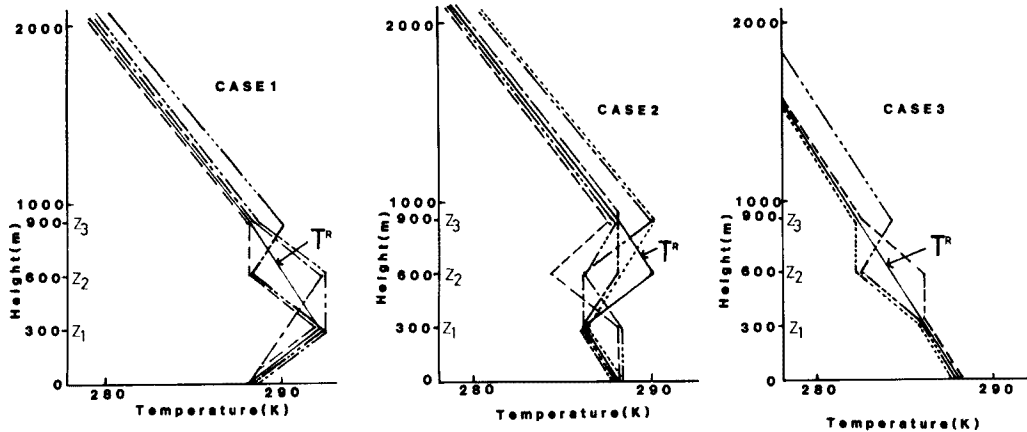
Fig. 2. Test results of the library method. Real temperature profiles ( T^R ) and estimated temperature profiles (difference of brightness temperature < 0.5 K).
