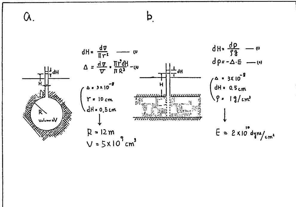
Fig. 4. Idealized models of the observation well. a: Well ending a finite cavity. b: Well drilled into a confined aquifer.
