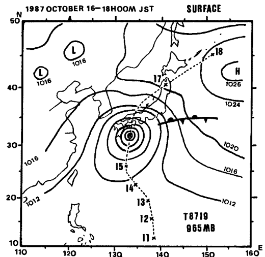
Fig. 11. Weather map (surface) at 18 h00mJST on 1987 October 16. Each cross shows the location of the center of the Typhoon 8719 at each 18 h00m of the days from October 11 to 18.
