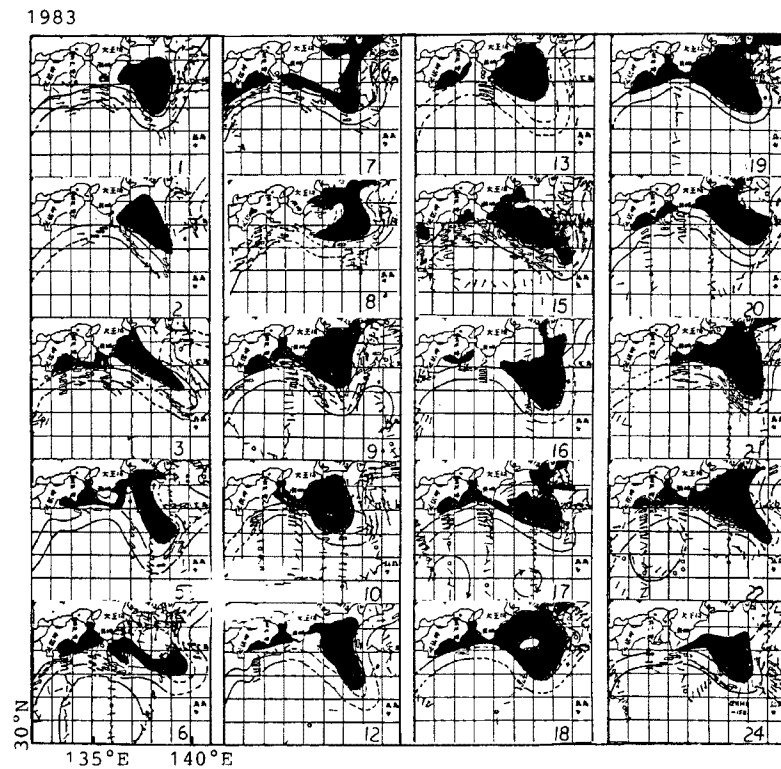
(h) ○ 0-0.2kn ← 0.3-0.9kn ← 1.0-1.9kn ← greater than 2.0kn ● less than 12°C at 200m depth
