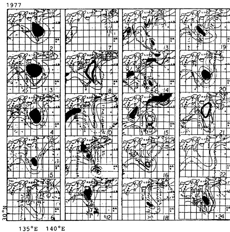
(b) ○ 0-0.2kn ← 0.3-0.9kn ← 1.0-1.9kn ← greater than 2.0kn ● less than 12°C at 200m depth
