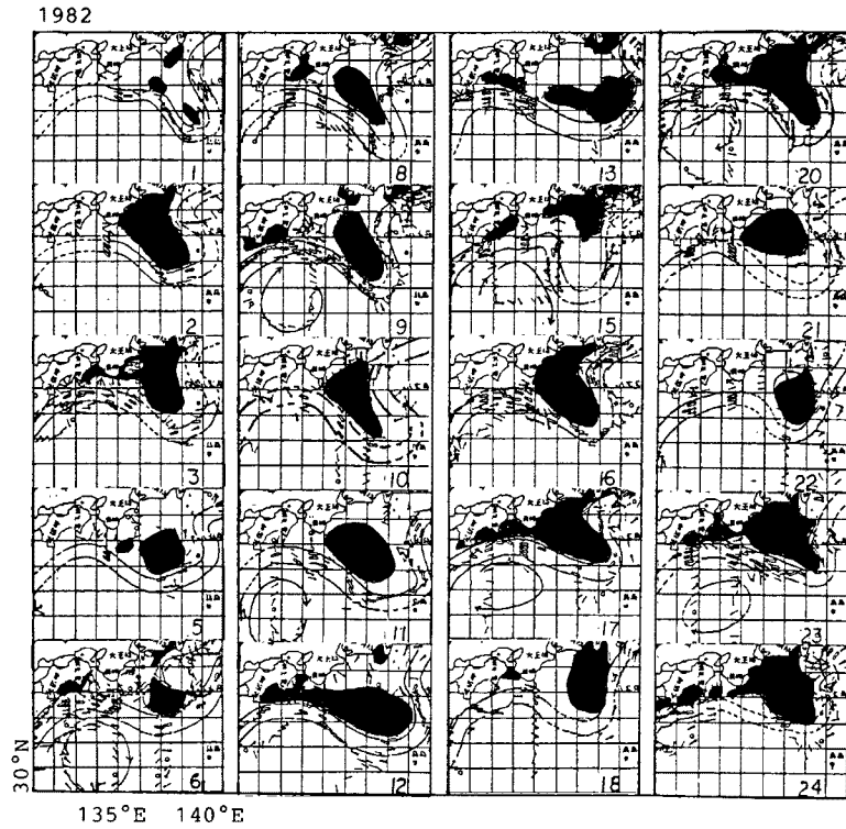
(g) ○ 0-0.2kn ← 0.3-0.9kn ← 1.0-1.9kn ← greater than 2.0kn ● less than 12°C at 200m depth
