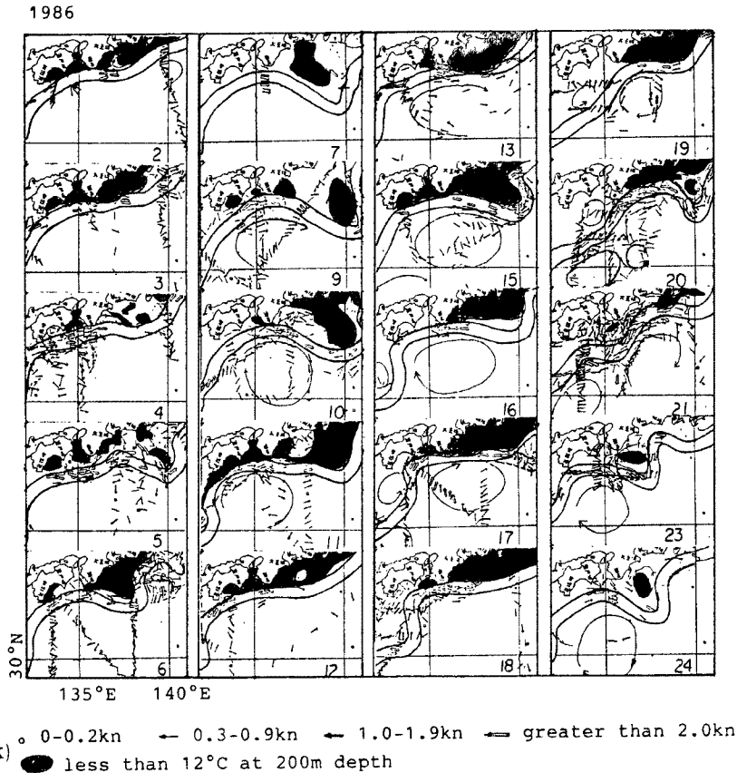
Fig. 4. Sequential map of the Kuroshio path and area where water temperature at 200 m depth is below 12°C. (a) 1976, (b) 1977, (c) 1978, (d) 1979, (e) 1980, (f) 1981, (g) 1982, (h) 1983, (i) 1984, (j) 1985, (k) 1986
