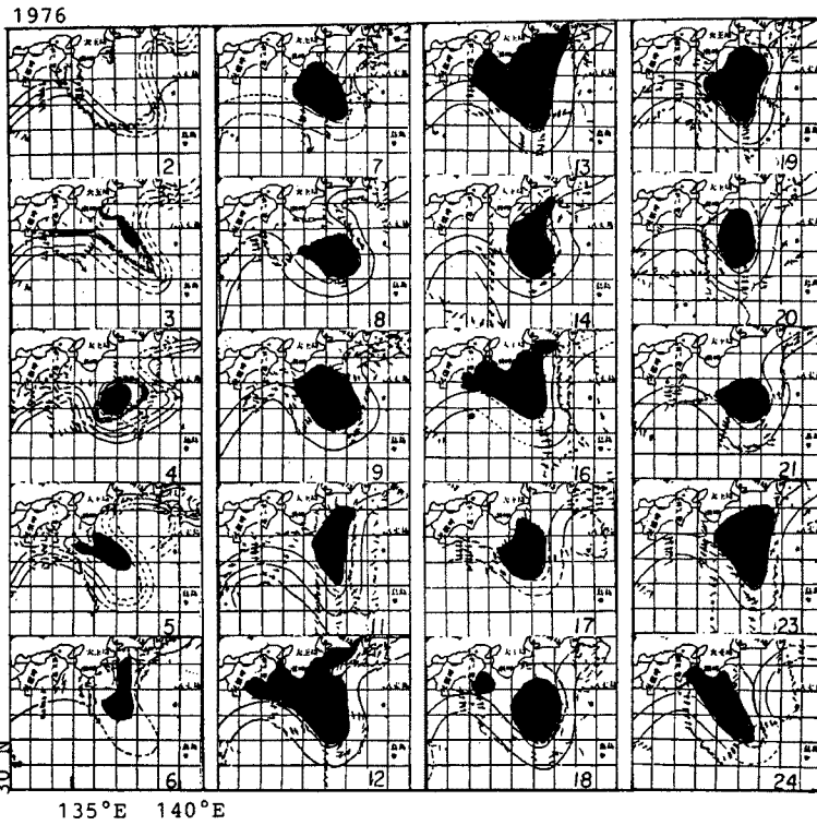
(a) ○ 0-0.2kn ← 0.3-0.9kn ← 1.0-1.9kn ← greater than 2.0kn ● less than 12°C at 200m depth
