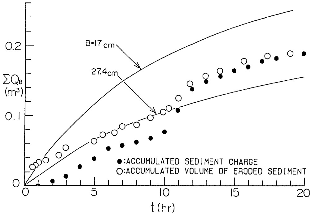
Fig. 15. Comparison between the calculated and experimental results for accumulated sediment discharge. In the calculation with one-dimensional governing equations, two stream widths predicted by present method ( B=17 cm) as well as by regime theory ( B=27.4 cm) are applied.
