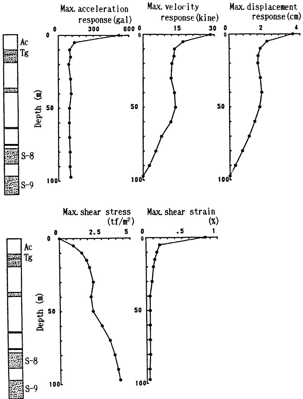
Fig. 3. Results of dynamic response analysis for a simplified model of Senshu-oki seabed
