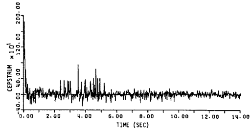
Fig. 10. Cepstrum of simulated displacement.
