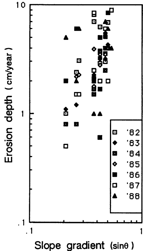
Fig. 3. Relationship between erosion depth ( E ) and slope gradient ( \theta ) on bare slopes.
