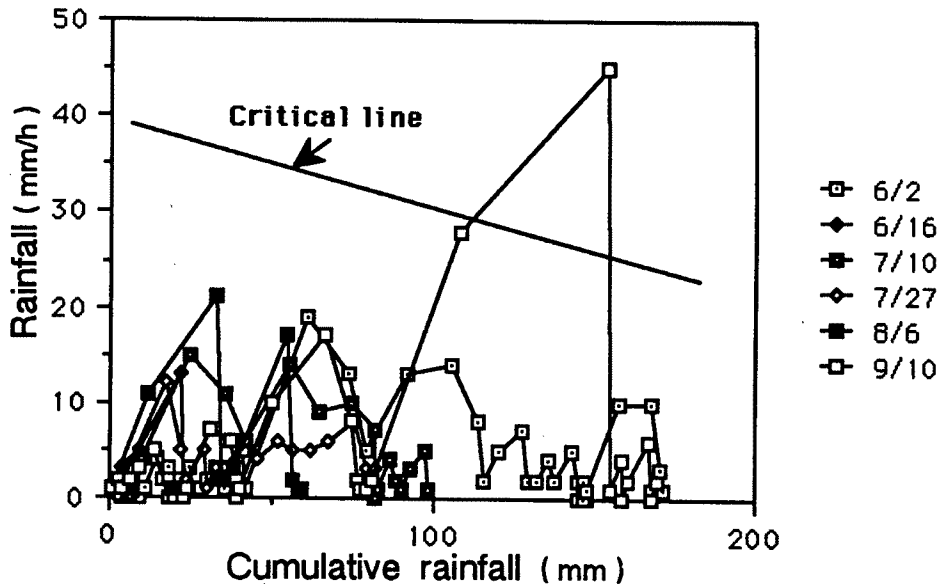
Fig. 16. Time sequential diagram of rainfall intensity and cumulative rainfall.
