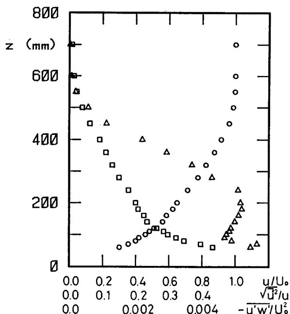
Fig. 4. Wind characteristics of approach flow at x=15.1 m, y=-0.155 m: ○, u/U_0 ; □, \sqrt{u'^2}/u ; △, -u'w'/U_0^2 .
