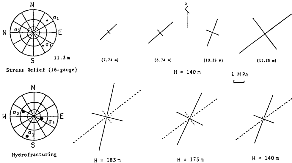
Fig. 5. Results of absolute stress measurements at Tsuchihashi site. Directions of principal stresses shown on stereographic net of lower hemisphere (leftmost) and the principal axes of horizontal stress (right). Upper: by stress relief method. Lower: by hydrofracturing method. The values in parenthesis are the depth of the measuring point from the mouth of borehole. H is the depth of measured point from the ground surface. Solid line shows the measured values, and broken line shows the principal stress values after correction, assuming the principal stress direction N52° E.
