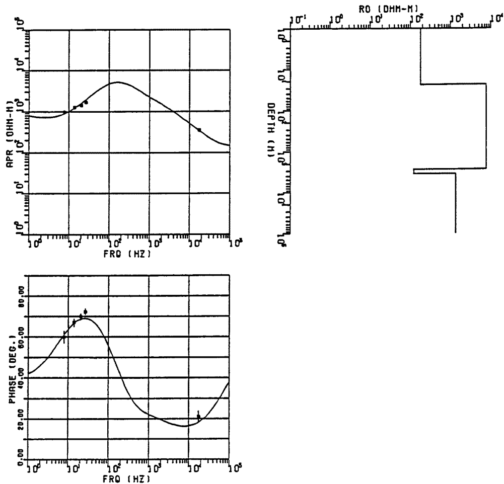
Fig. 5. Calculated apparent resistivity and phase based on a four layered model. The upper figure on the left-side shows the apparent resistivity and the lower figure shows the phase angle. Solid squares indicate the observed values and the solid lines indicate the calculated values based on the resistivity model shown on the right side.
