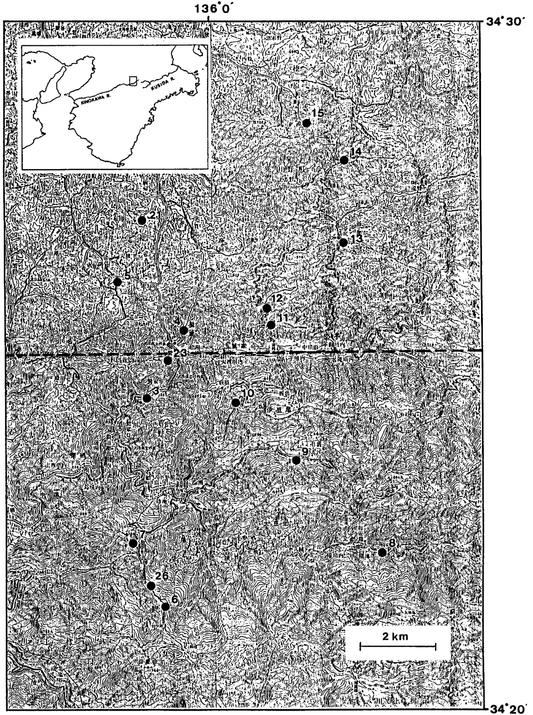
Fig. 1. Observation sites. Solid circles indicate observation sites and figures beside circles show site numbers. Thick broken line indicates the Median Tectonic Line (MTL) inferred from the surface geological map.
