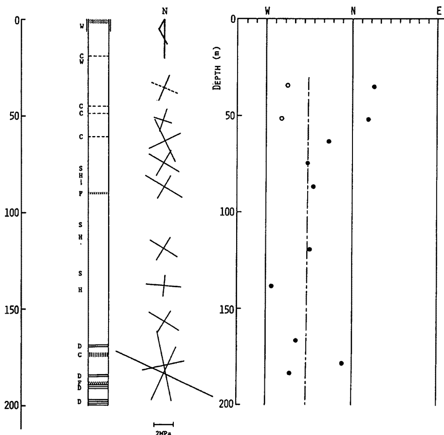
Fig. 3. Left: columnar section of borehole. C: crack, F: fracture, D: discing, S: soft, H: hard, W: weathered Middle: principal stress axes in horizontal plane at each depth. Right: azimuths of maximum principal stress at each depth. ○: estimated maximum stress azimuth after excluding topographical effects.
