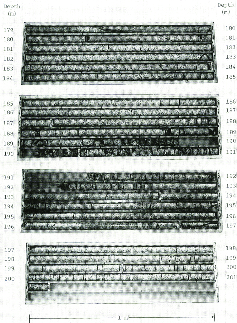
Photo. 1. Boring core taken at Mannari measuring site (Depth: 179~201.1m). Discing phenomena are clearly seen on cores deeper than 190m.
