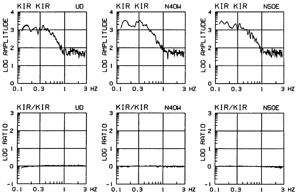
Fig.7. Comparison of velocity seismograms of microtremors, velocity amplitude spectra and spectral ratios obtained with different instruments at the same site. Note the same wave forms and spectra showing the accurate instrumental corrections.
