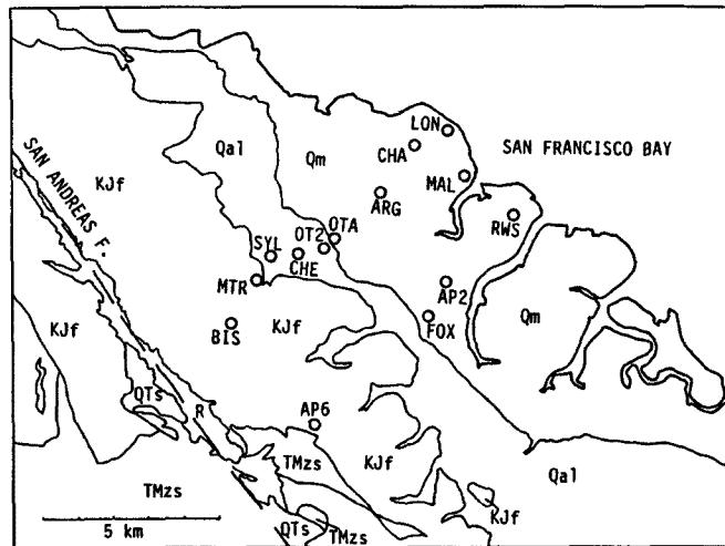
Fig. 2. Surface geology and site locations in Peninsula Cities. Notations of geology are ; KJf=Franciscan formation, TMzs=Tertiary Mesozoic sedimentary rocks, Qa1=Quaternary alluvial deposits, and Qm=fill on baymud.
