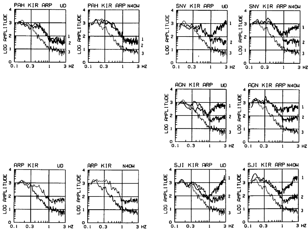
Fig. 12. Amplitude spectra and their variation with site locations in Santa Clara Valley. Vertical components and horizontal components in the direction parallel to the longitudinal axis of the bay ( N40^\circ W ) are shown. 1: ground site, 2: KIR, 3: ARP.
