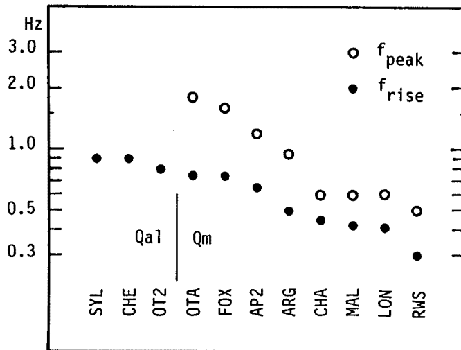
Fig. 10. Spatial variation of characteristic frequency for soil amplifications. f_{peak} = peak frequency of spectra at soil sites, f_{rise} = frequency at which amplification occurs.
