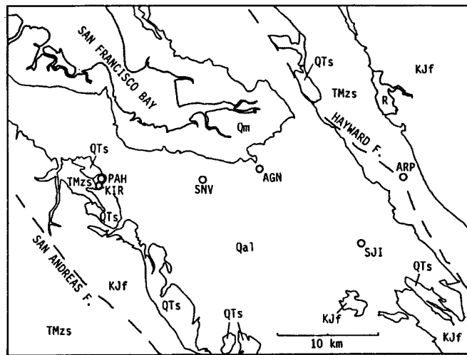
Fig. 4. Surface geology and site locations in Santa Clara Valley. Notations of geology are the same as those in Fig. 2.
