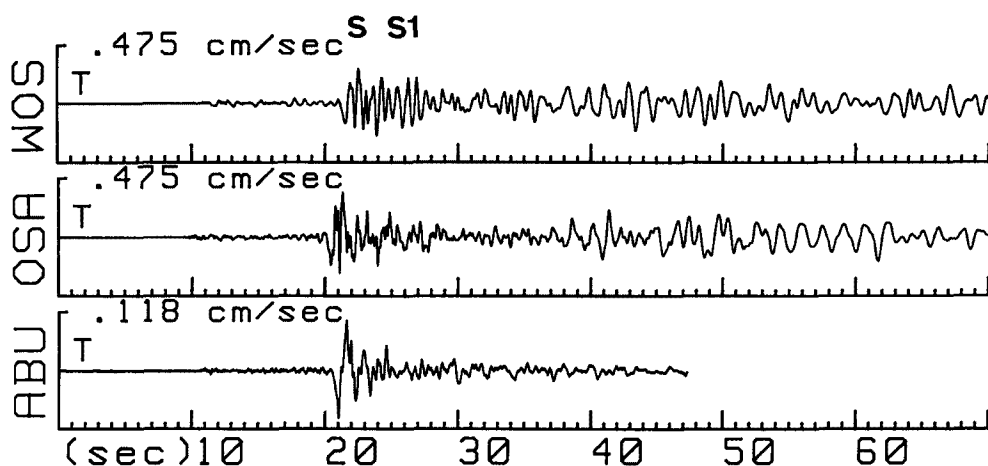
Fig. 7. Comparison of wave forms observed at WOS (soft soil site), OSA (hard ground site) and ABU (rock site) for the earthquake (No.3) in the central part of Mie prefecture. Traces are transverse components (T) of particle velocity. Principal part of a S wave at WOS is elongated by the superposition of a reflected S wave on the S-wave coda. S-wave form at OSA is similar to that at ABU and also the duration of S-part is short compared with the duration at WOS.
