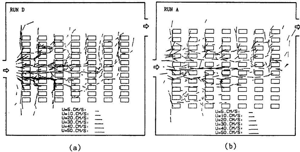
Fig. 12. Distribution of surface flow vectors. (a): RUN D (b): RUN A
