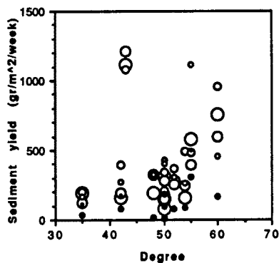
Fig. 4. Relation between the gradient ( \theta ) of bare slope and the rate of sediment yield (gr./m 2 /week).
