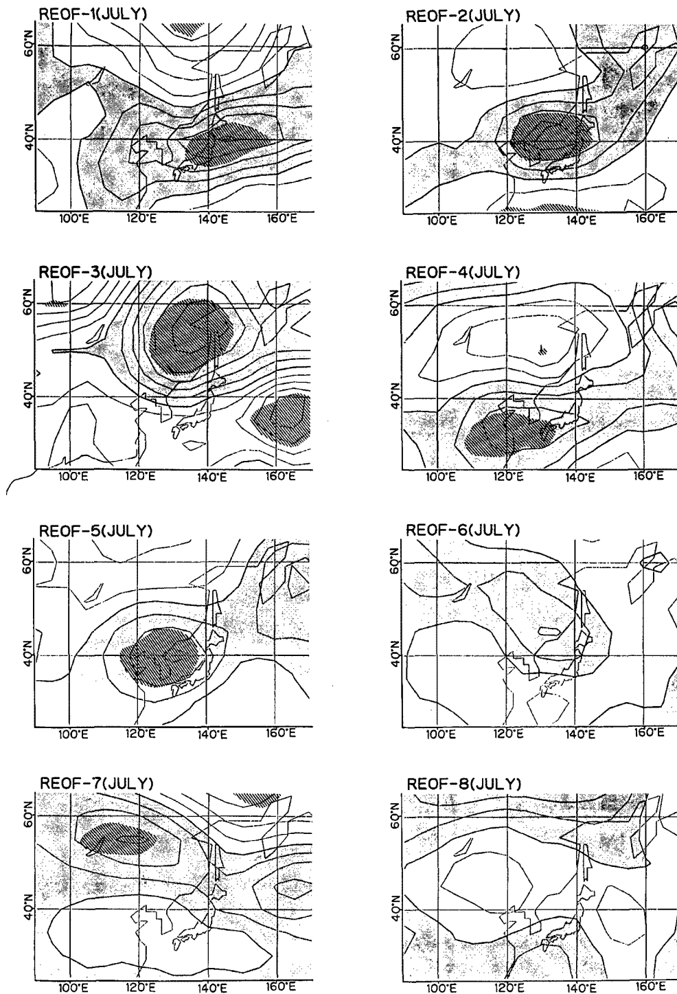
Fig. 13. Same as Fig. 9, except for July.
