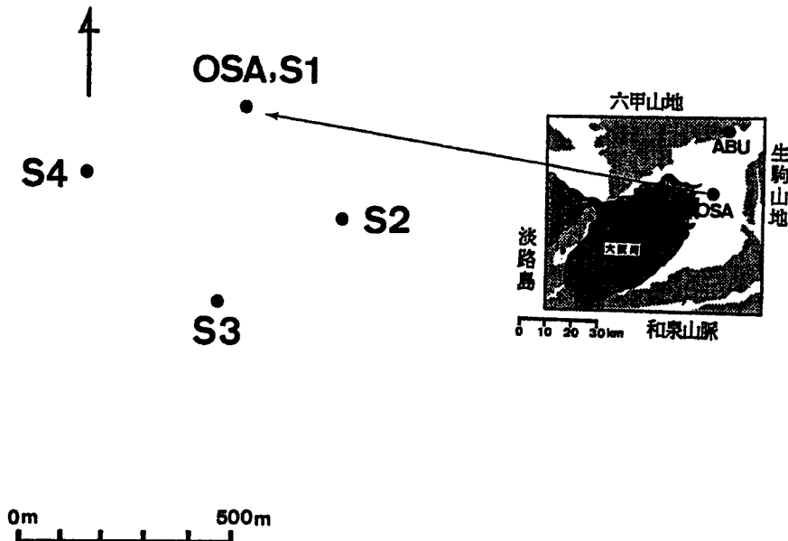
Fig. 2. Location of small seismic array deployed in the central Osaka Plain. The array is composed of four stations (S1 to S4) located around OSA. The aperture of the array is about 600 m.
