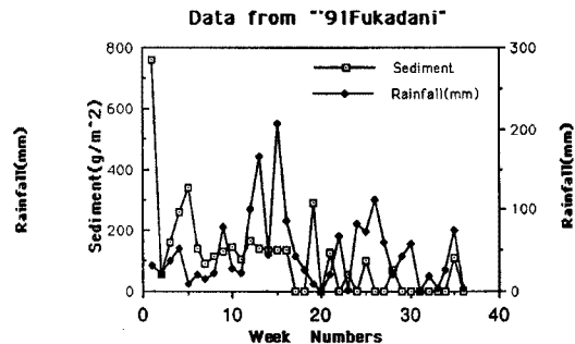
Fig. 6. Relation between rainfall ( \text{mm/week} ) and the rate of sediment yield ( \text{gr./m}^2/\text{week} ) at No. 7 site.
