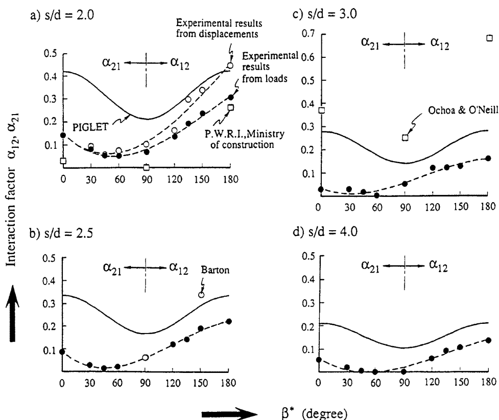
Fig. 14. Relationship between interaction factors \alpha_{12} , \alpha_{21} and the angle from the loading direction of piles \beta^* .
