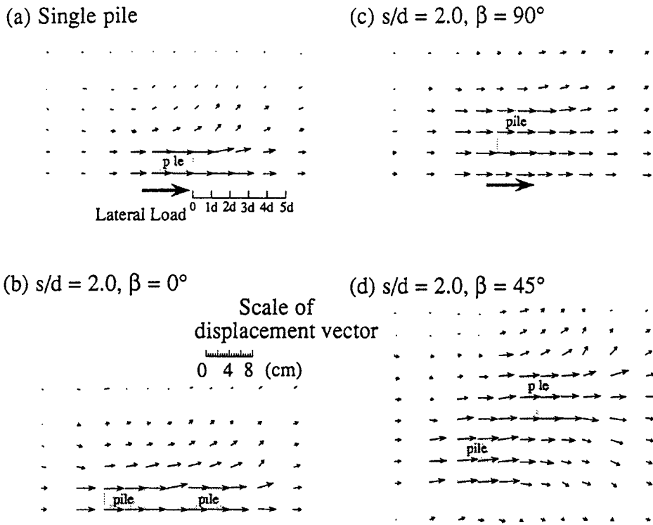
Fig. 21. Displacement vectors of the ground surface ( \delta/d=0.10 ).
