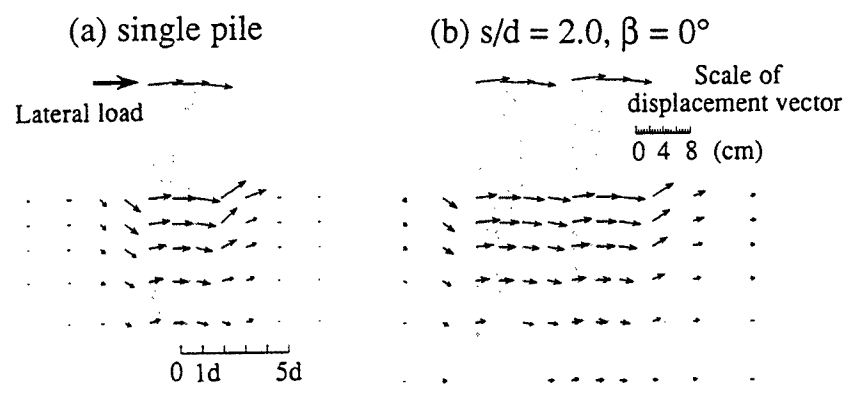
Fig. 22. Displacement vectors of the symmetric plain ( \delta/d=0.10 ).
