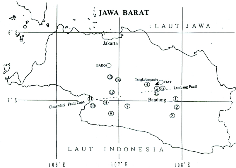
Fig. 1 GPS network in west Java. CIAT and BAKO are GPS stations at Ciatri and BAKOSURTANAL in Cibinong, respectively. 1: Nagreg, 2: Leles, 3: Garut, 4: Cikalongwetan (TTG. 95), 5: Lembang, 6: Cibodas, 7: Sukanegara, 8: Sagaranten, 9: Bojonglopang, 10: Kiaradua (LIPI), 11: Pelabuhanratu, 12: Cisaat, 13: Ciawi, 14: Tugu, 15: ITB1.
