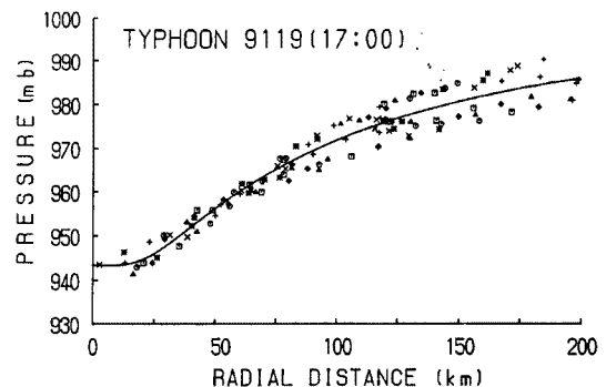
Fig. 5 Same as Fig.3, except for Typhoon 9119, at 17:00JST, Sept.27, 1991 (from Fujii, Hayashi and Mitsuta 9) )
