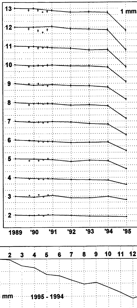
Fig. 2. Upper: Changes of baseline Lengths referred to site 1 in 1989 - 1995. Lower: Change of baseline lengths in 1994 - 1995.
