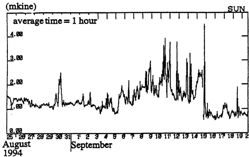
Fig. 2. Amplitude variations of volcanic tremors (25 Aug. 1994–20 Sep. 1994)
