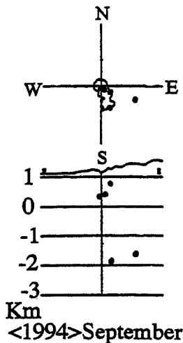
Fig. 13. Distribution of volcanic earthquakes in September 1994
