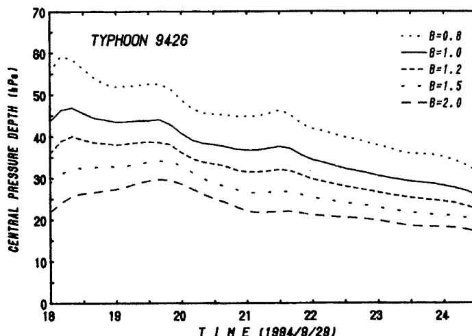
Fig. 18. Same as Fig. 12, except for \Delta p
