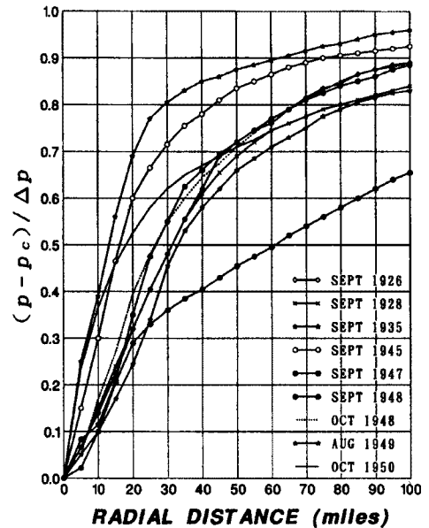
Fig. 1. The radial pressure distributions of nine hurricanes investigated by Schloemer 1)
