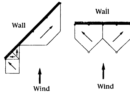
Fig. 13. Flow calculated with 2-D potential flow theory along a wall.
