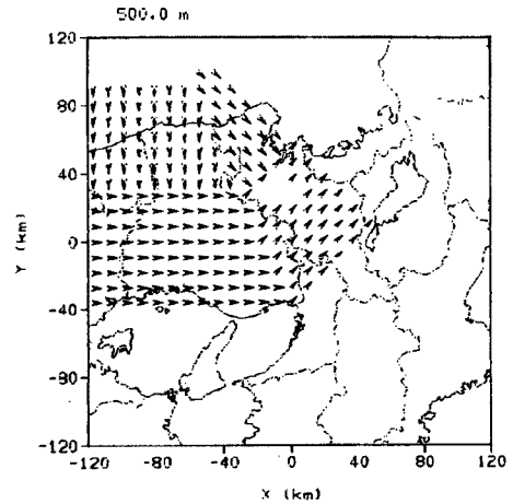
Fig. 11. Initial wind inferred along the front.
