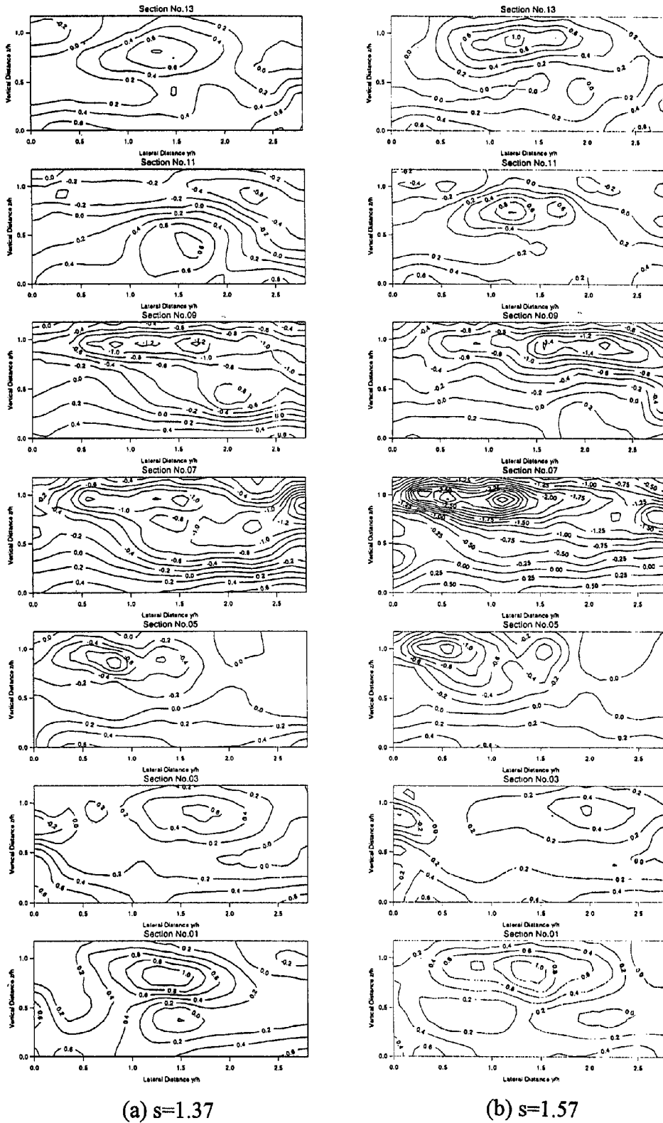
Fig. 5 Reynolds stress -\overline{uu'}/u_*^2 for the overbank flow, Dr = 0.15 , (a) s = 1.37 (left) and (b) s = 1.57 (right)
