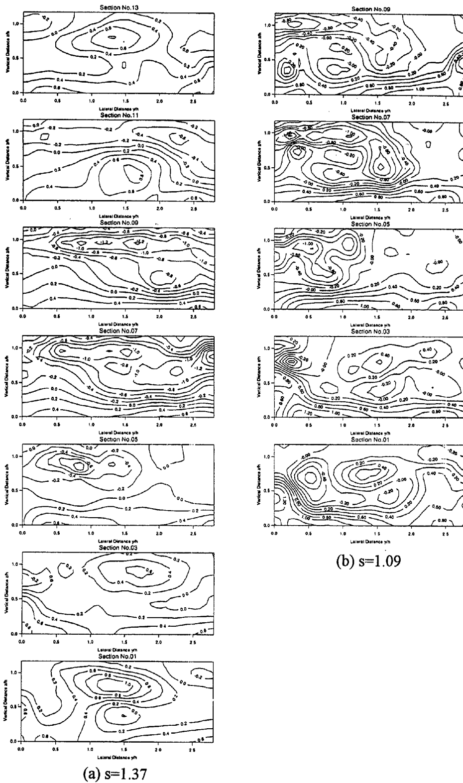
Fig. 9 Reynolds stress -\overline{uu'}/u_* for the overbank flow, Dr = 0.15 , (a) s = 1.37 (left) and (b) s = 1.09 (right)
