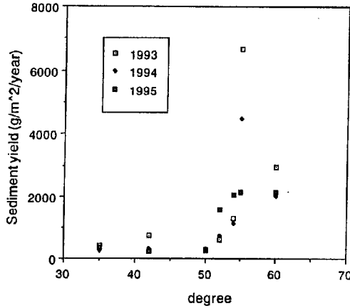
Fig. 13 Relation between the rate of erosion ( \text{g}/\text{m}^2/\text{year} ) and the gradient of slope
