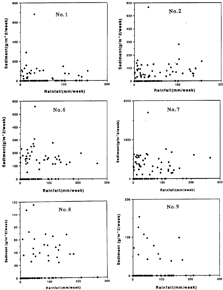
Fig. 12 Relation between rainfall (mm/week) and the rate of erosion ( \text{g}/\text{m}^2/\text{week} ) in the experimental plots
