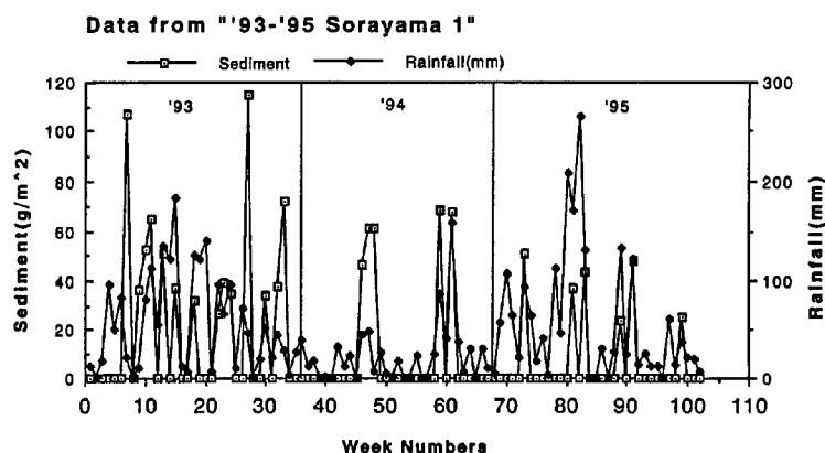
Fig. 7 Hysteretic characteristics of the rate of erosion (g/m 2 /week) and rainfall (mm/week) on the experimental plot No.8
