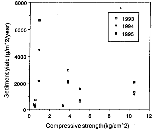
Fig. 14 Relation between the rate of erosion ( \text{g}/\text{m}^2/\text{year} ) and the compressive strength ( \text{kg}/\text{cm}^2 )
