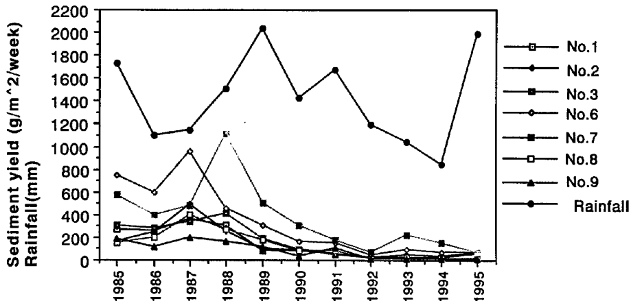
Fig. 15 Hysteretic characteristics of the rate of erosion ( \text{g}/\text{m}^2/\text{year} ) and rainfall (mm) on the experimental plots
