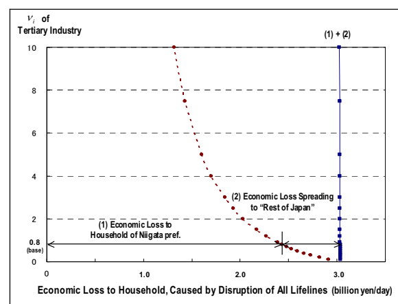
Fig. 7 Sensitivity Analysis on Substitution Parameter v_i
