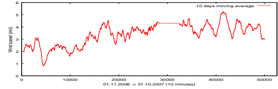
Wind Velocity (10 day average)
