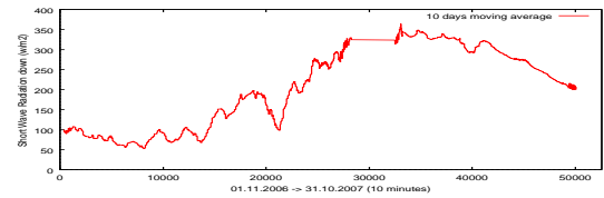
Shortwave Radiation (Down, 10 day average)
