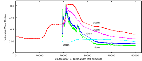
Volumetric Water Content (VWC)
