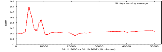
Albedo (10 day average)
