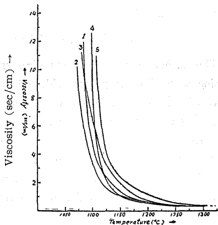
Fig. 2. Viscosity-temperature curves.
