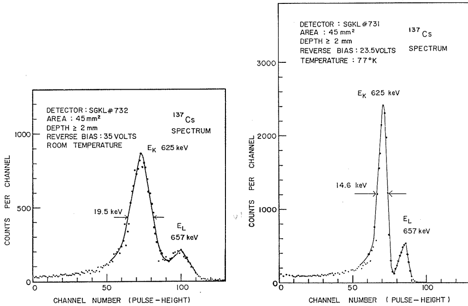
Fig. 7. Pulse-height spectrum of conversion electrons of ^{137}\text{Ba} observed with a p-i-n silicon junction detector at room temperature.
