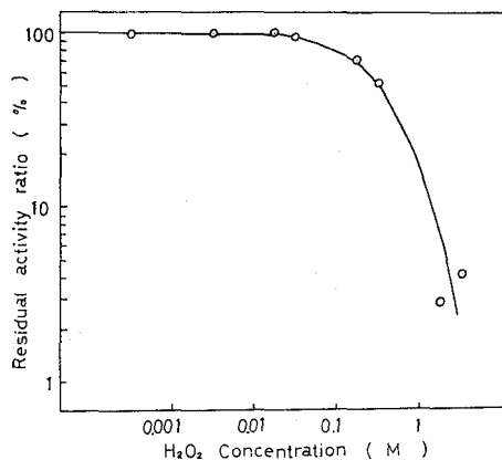
Fig. 3. Effect of H_2O_2 on \alpha -amylase activity.
