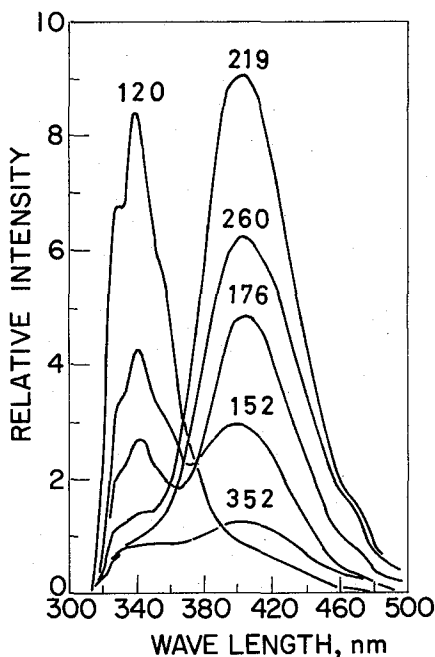
Fig. 6. Temperature dependence of fluorescence spectra of 10^{-3} M solutions of poly(1-vinylnaphthalene) in 2-methyltetrahydrofuran (after David et al. 24) . Concentration in units of naphthalene rings.
